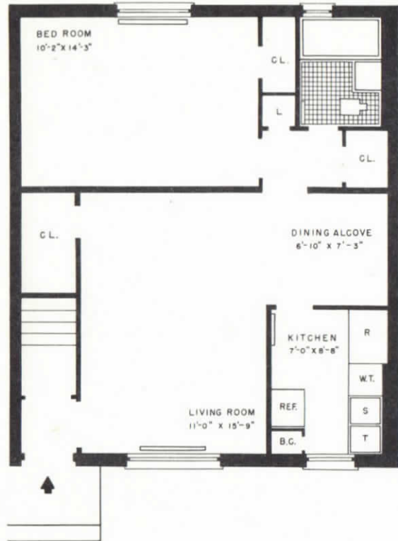
3 1/2 ROOM APARTMENT FIRST FLOOR
