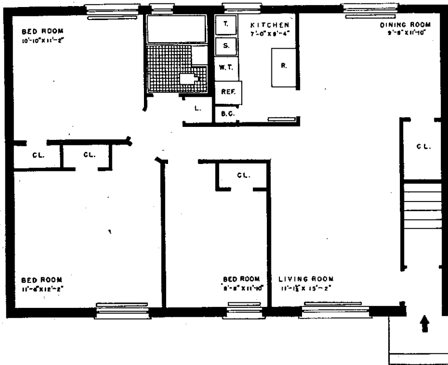
6 ROOM APARTMENT FIRST FLOOR
